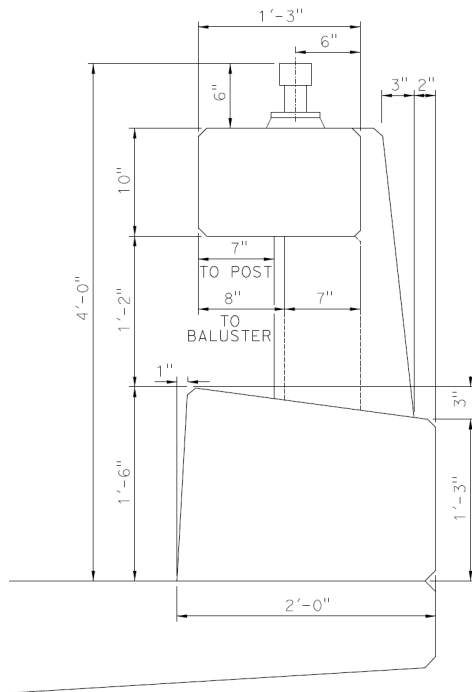
Figure 1 Typical Section of Concrete Barrier Type 86H
