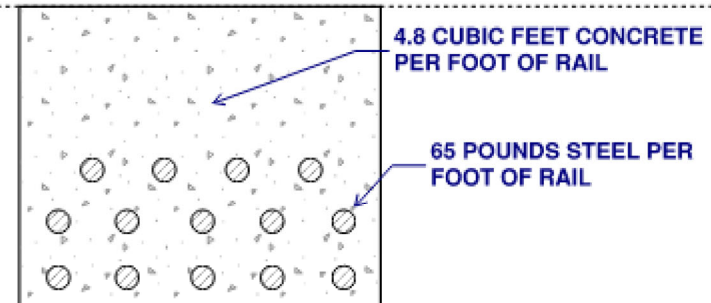
NEW STANDARD TYPE 86H RAIL
