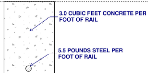
OLD NOJOQUI CREEK BRIDGE BALLUSTER RAIL
