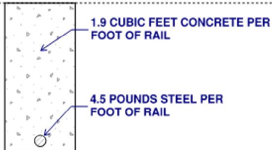
EXISTING GARRAPATA CREEK BRIDGE BALLUSTER RAIL
