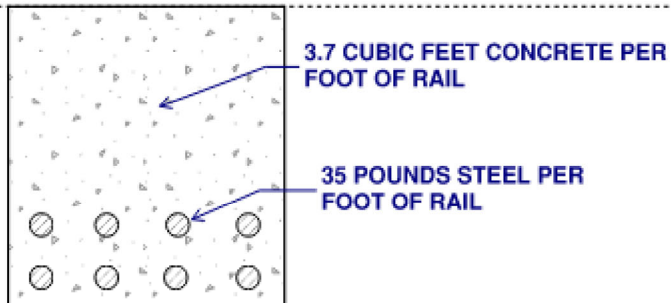
UPGRADED NOJOQUI CREEK BRIDGE TYPE 80 RAIL
