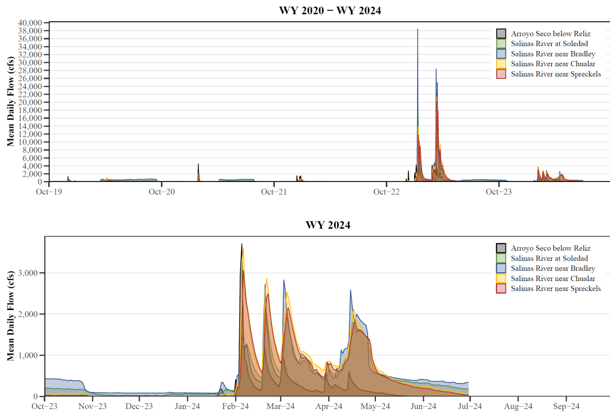
Mean Daily Flow at select Salinas River and Arroyo Seco USGS Streamflow Gages
