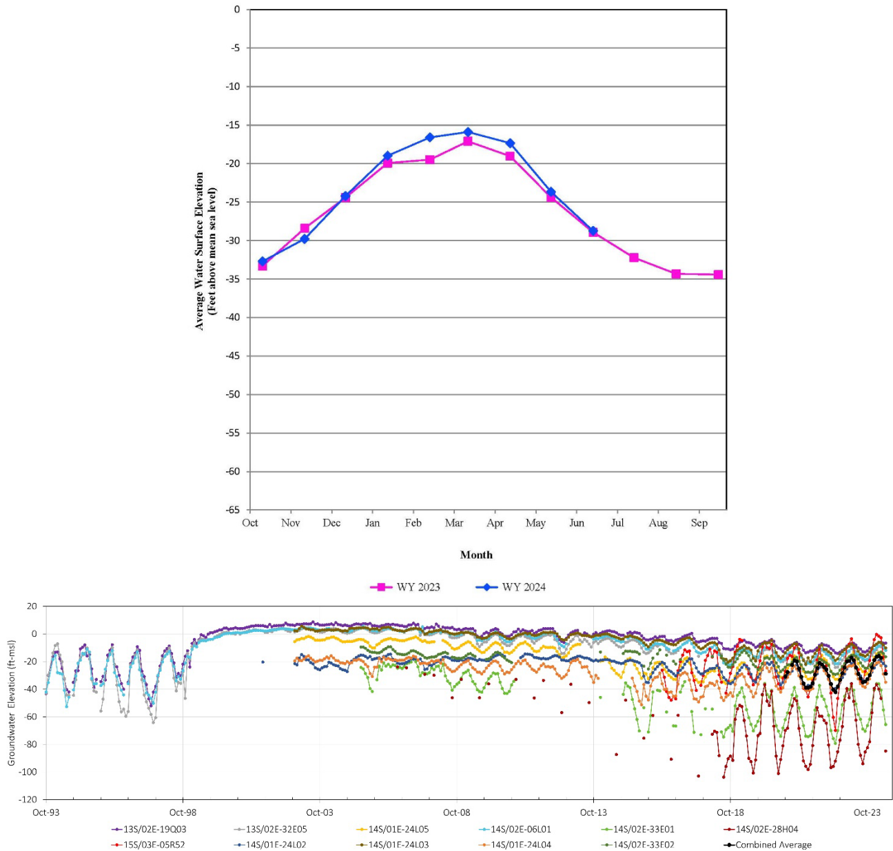
Figure 9: Groundwater Elevation Trends in the Deep Aquifers
