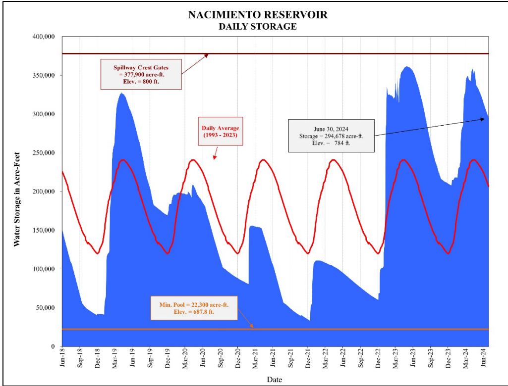
Figure 4: Nacimento Reservoir Storage
