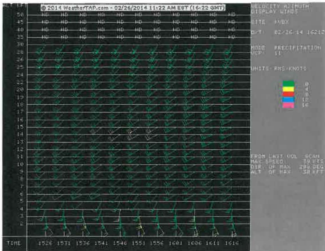
Figure 5.4 Vandenberg AFB Doppler winds, 0726-0816 PST, February 26, 2014
