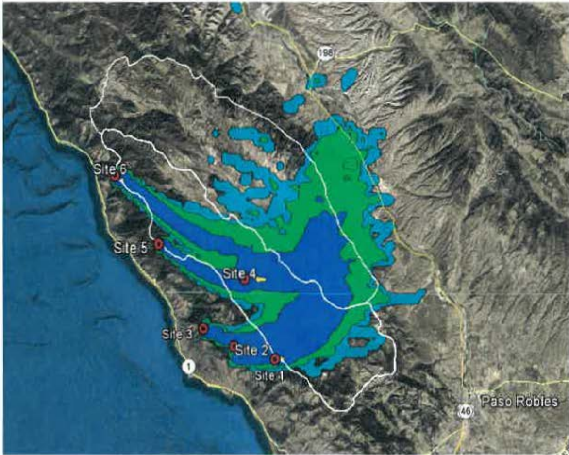
One-hour HYSPLIT simulation for a storm period on December 12, 2014
