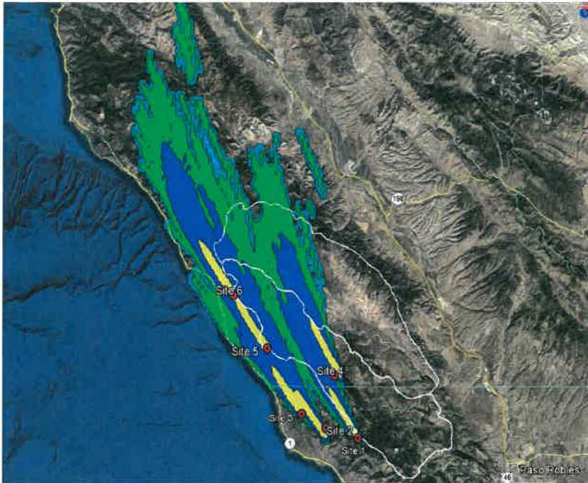
One-hour HYSPLIT simulation of seeding material plumes for possible ground generator locations for a storm period on December 5, 2010; in these plots, yellow (if present) represents the highest concentration of seeding material near the center of the plume; dark blue areas have the next highest concentration, followed by green and light blue shading which depict the weaker concentrations near the edges of the plumes.
