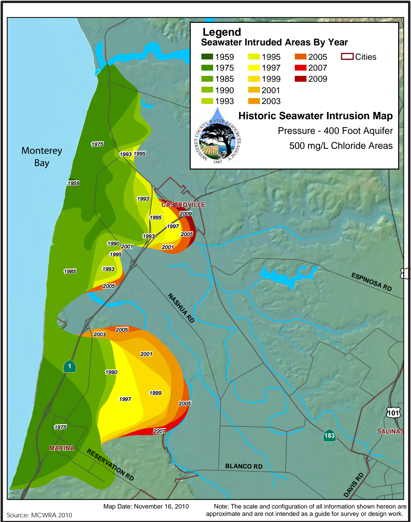
FIGURE 3.6-5B HISTORIC SEAWATER INTRUSION MAP - 400-FOOT AQUIFER
