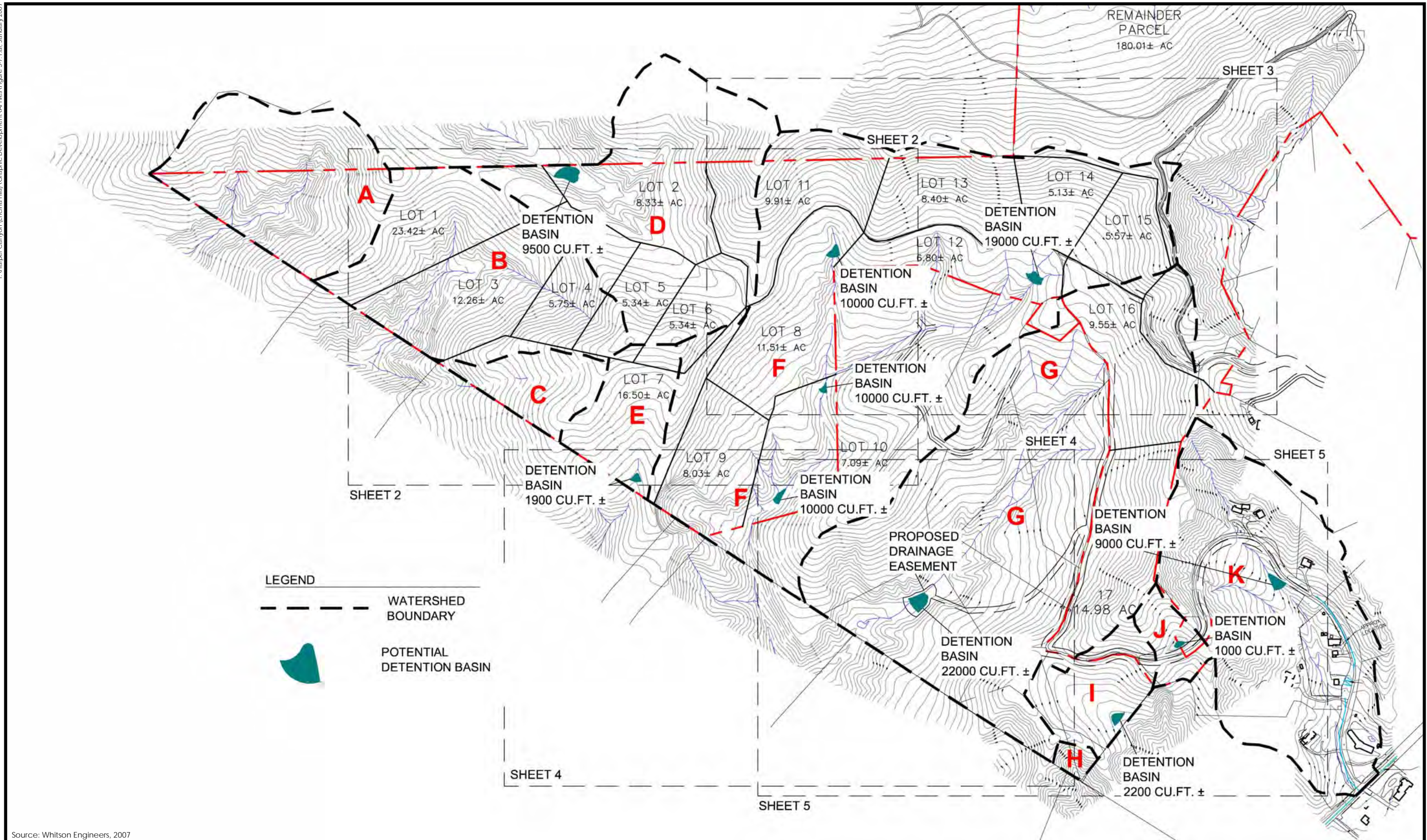
FIGURE 3.7-1 WATERSHED AND PROPOSED DETENTION BASINS
