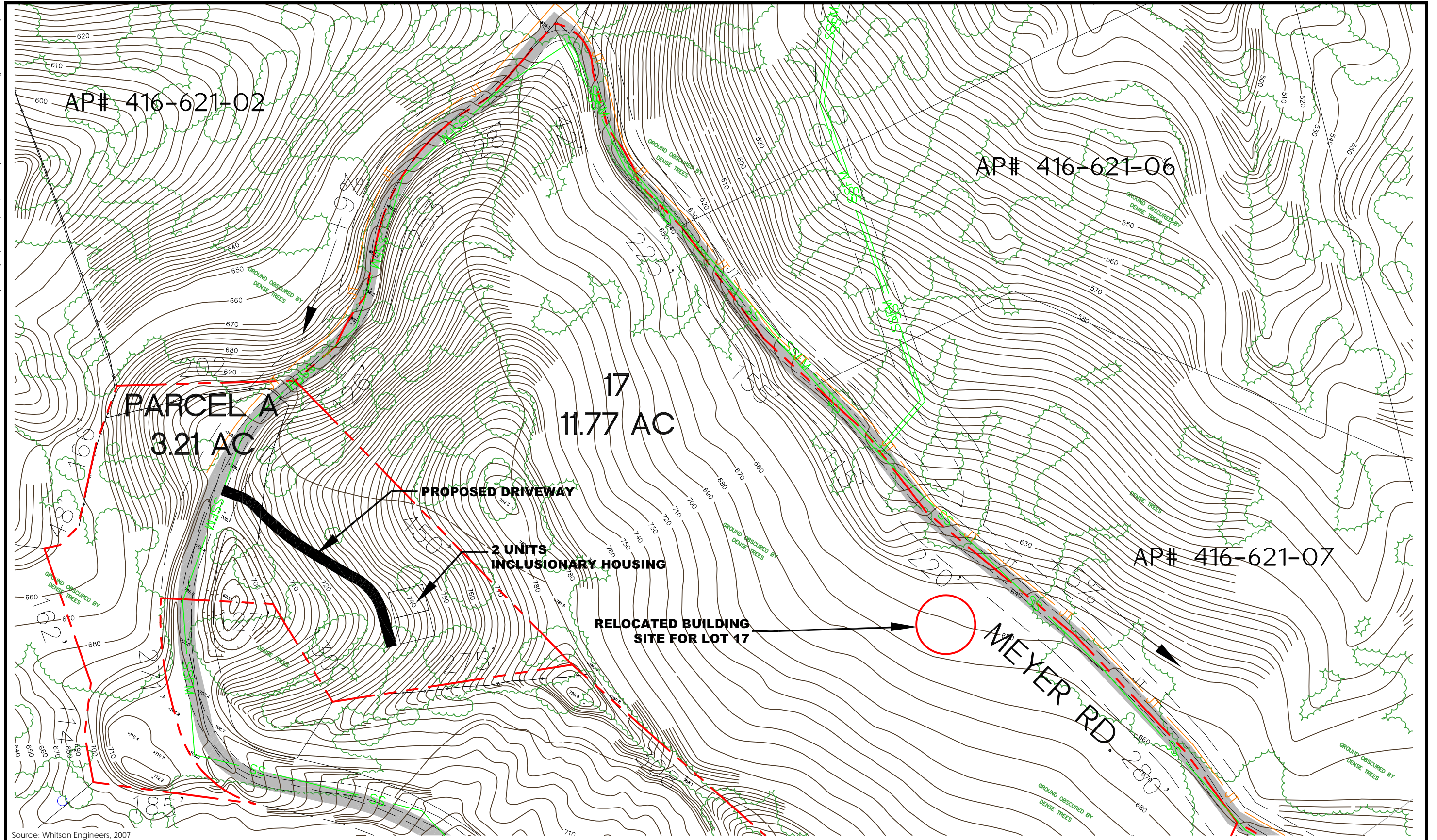
FIGURE 4.1 MODIFIED SUBDIVISION DESIGN 'A' PMC
