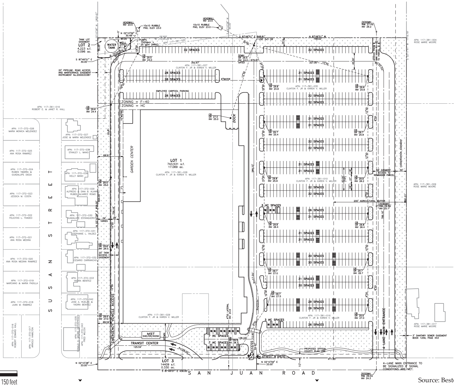
Figure 5 Proposed Commercial Project Site Plan Miller Trust Commercial EIR Notice of Preparation
