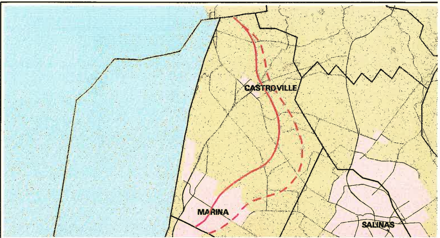
Figure 1-46a. 500 ppm Chloride Contour, 180-Foot Aquifer, Historical and Without Reservoir Simulation. September 1994
